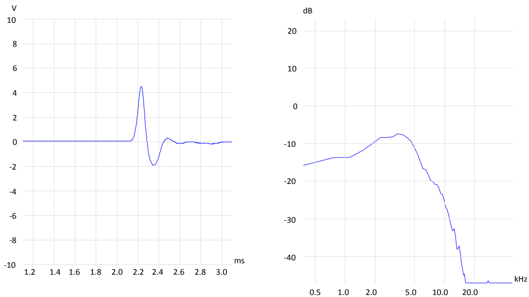
Figure 1 - Boomer Pulse and Frequency Spectrum, 3m, 480J, -189.25 dBV re 1 \mu Pa sensitivity
